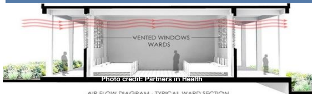
AIR FLOW DIAGRAM - TYPICAL WARD SECTION
